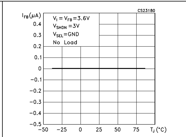
Figure 11. Current feedback leakage vs temperature
